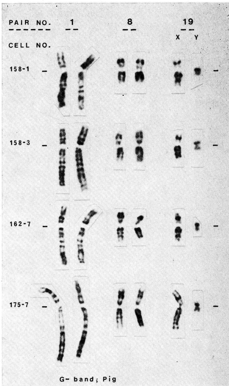
FIG. 1. — Chromosome pair Nos. 1, 8, and 19 (the sex chromosomes) from four pig leucocytes in three different metaphase stages. Cell 158-1 shows chromosomes contracted, cells 158-3 and 162-7 medium contracted, and cell 175-7 long chromosomes.
